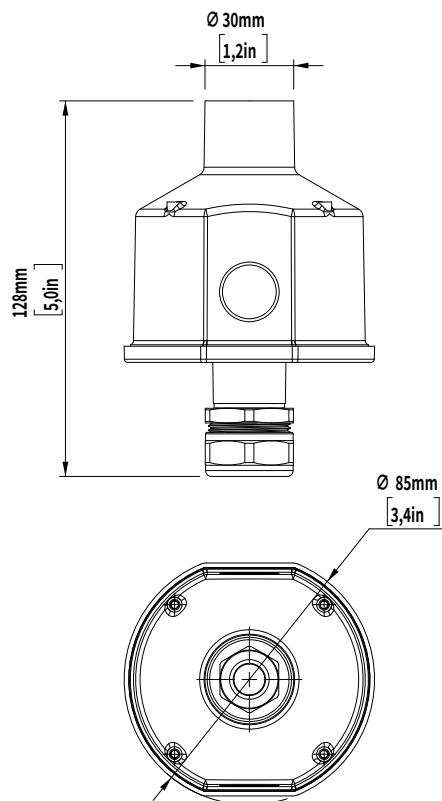
Technopolymer installation housing
