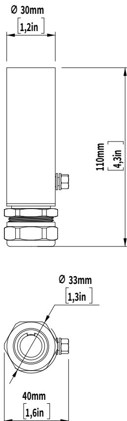
Stainless steel installation housing
